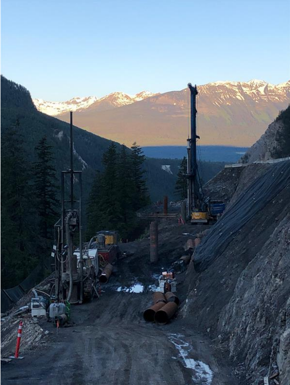
Figure 6: Wolf Viaduct – Pile installation ongoing – June 30, 2022
