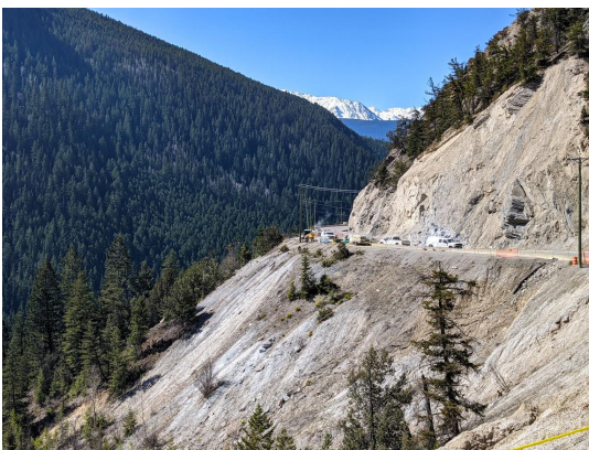
Bighorn Bridge April 2021: Drilling anchors
